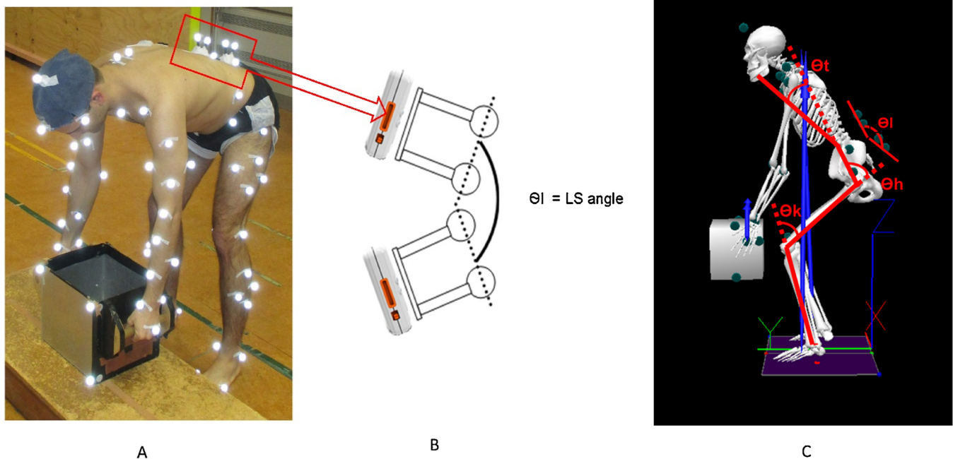
Fig. 1. A participant performing the lifting task (A). Real-time biofeedback on lumbar posture was provided by two inertial sensors attached to the lumbar spine (B). Two pairs of reflective markers attached to the sensors provided additional kinematic measures of lumbosacral (LS) angle (B). Relative joint angles ( \Theta_l = lumbosacral angle; \Theta_t = trunk angle; \Theta_h = hip angle; \Theta_k = knee angle) and joint moments (knee, hip and back) were calculated using a fifteen segment, rigid-link, dynamic biomechanical model and external ground reaction forces (C).
